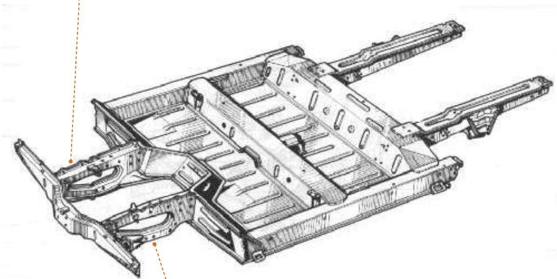
512895 MOTOR BEAM FRONT RIGHT
