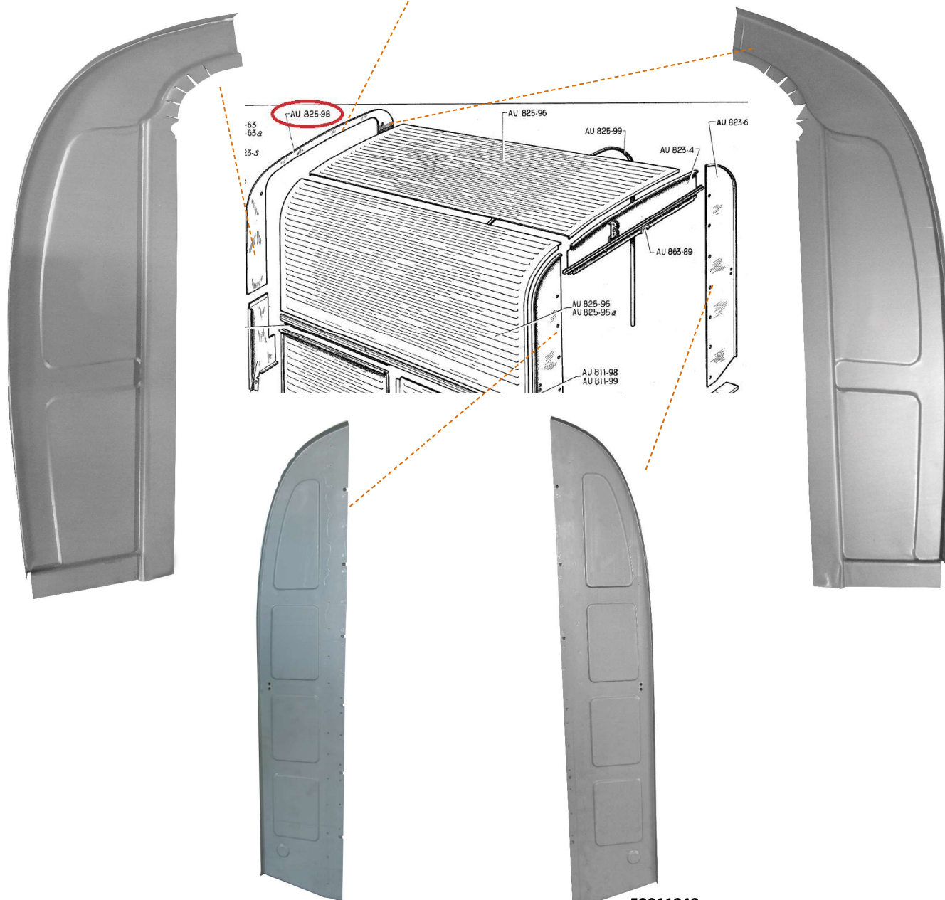
52011342 REAR LOCKPLATE LEFT AK250 / AZU
