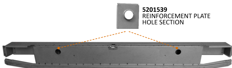
5201599 REAR VALANCE COMPLETE 2 HOLES
