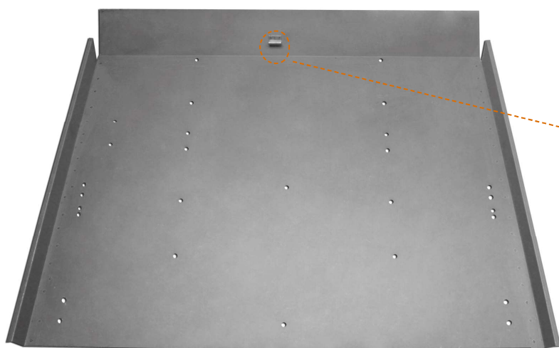
523090 FRONT FLOORPANEL
